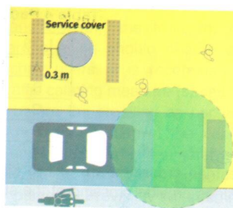
Fig. 45 Detail of Warning Tiles around Service Cover when provided on Walking Zone (Top View)
