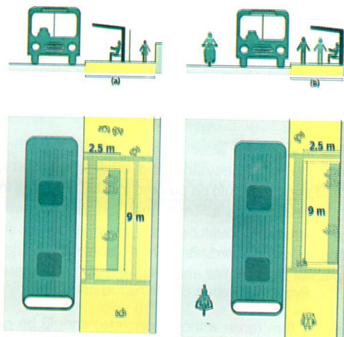
Fig. 51 Placement of Bus-Stop on Footpath (Top View)
