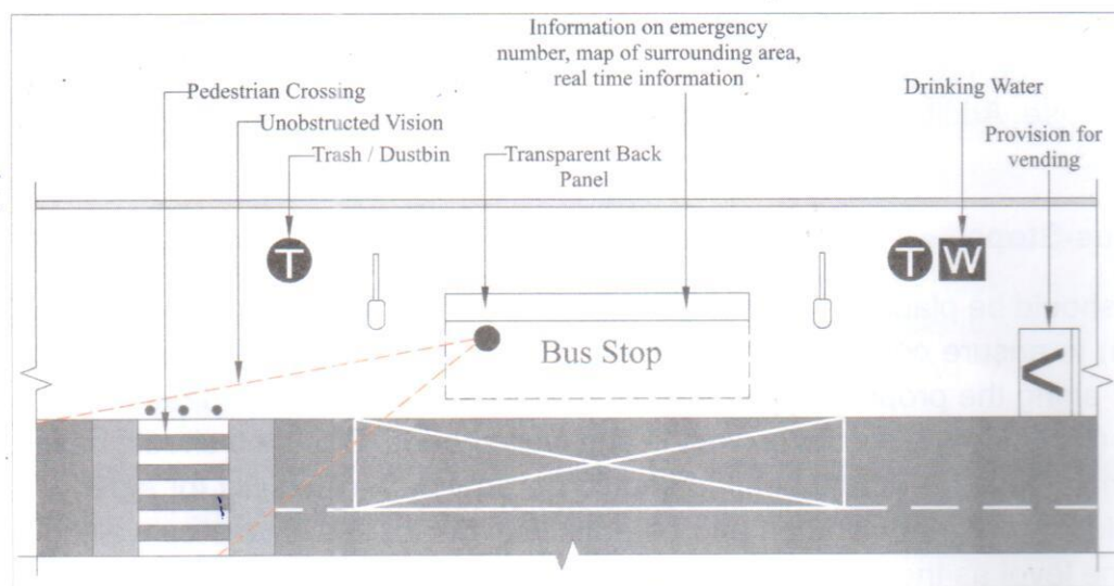
Fig. 52 Bus-Stop Area Planning (Top-View)
