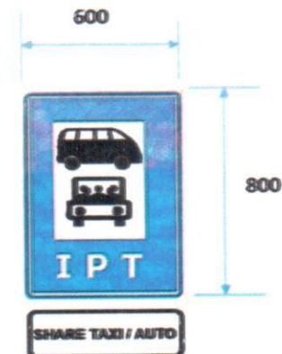
Fig. 90 Informal Public Transport Stop Signage
