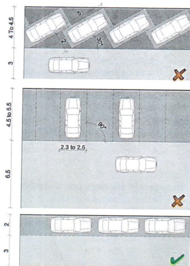
Fig. 56 Parallel Parking is preferred for all 3 & 4 Wheeler Vehicles
