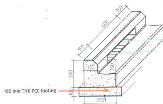
Fig. 27 Kerb Stone Block with Saucer Drain
