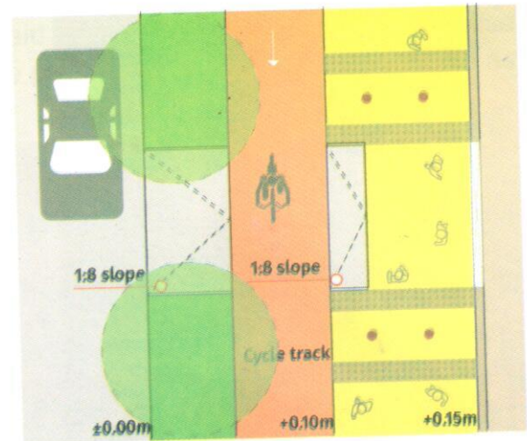
Fig. 21 Planning detail between Footpath and Cycle Track (Top View)
