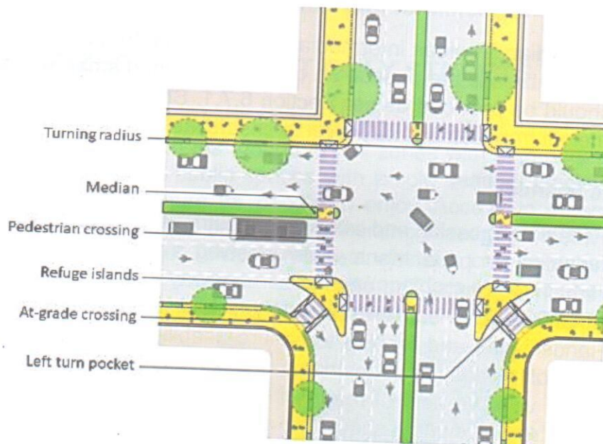
Fig. 63 Safe Intersection Design
