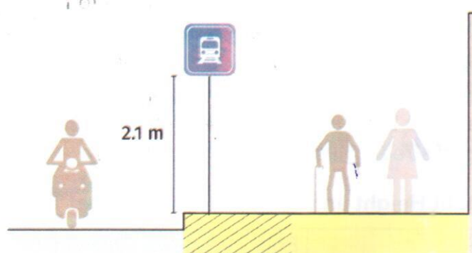
Fig. 37 Signage Placement on Footpath
