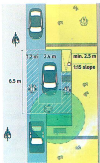
Fig. 59 On-Street Accessible Parking (Top-View)
