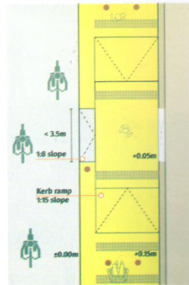
Fig. 17 Detail of Property Access on Small Footpath Widths (Top View)
