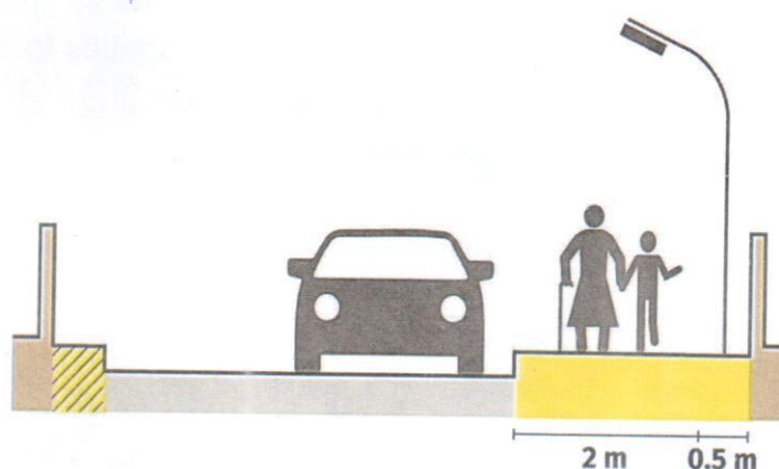
Fig. 11 One-Side Footpath on Narrow Streets
